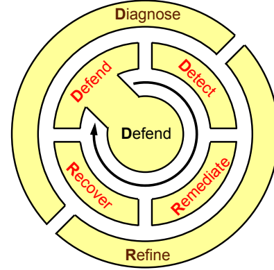
Fig. 1 ResiliNets strategy
