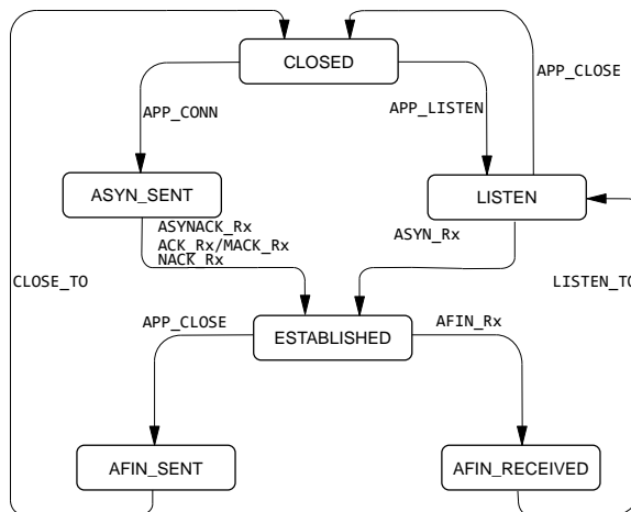
Figure 2: AeroTP state transition diagram
