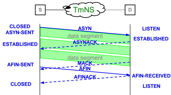
Figure 1: AeroTP connection management
