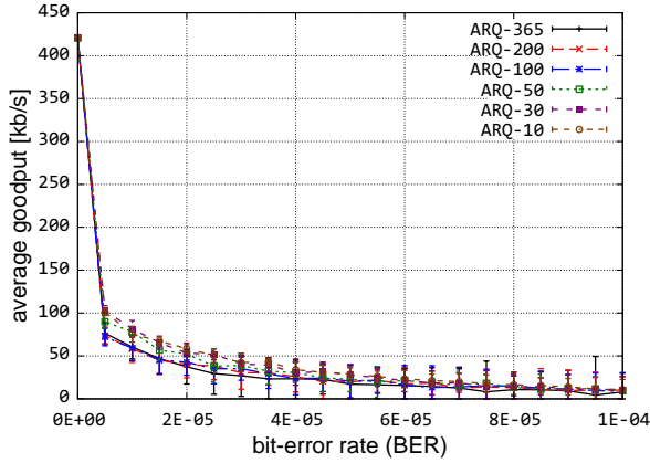
Figure 4: Fully reliable: Average goodput
