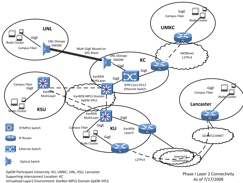
Fig. 10. GpENI current network connectivity. Source: https://wiki.ittc.ku.edu/gpeni/Image:GpENI-L2.png .
