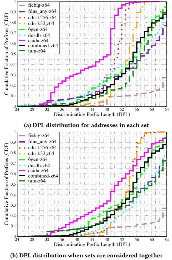
Figure 3: Discriminating Prefix Length (DPL) Distributions for target sets (CDF)
